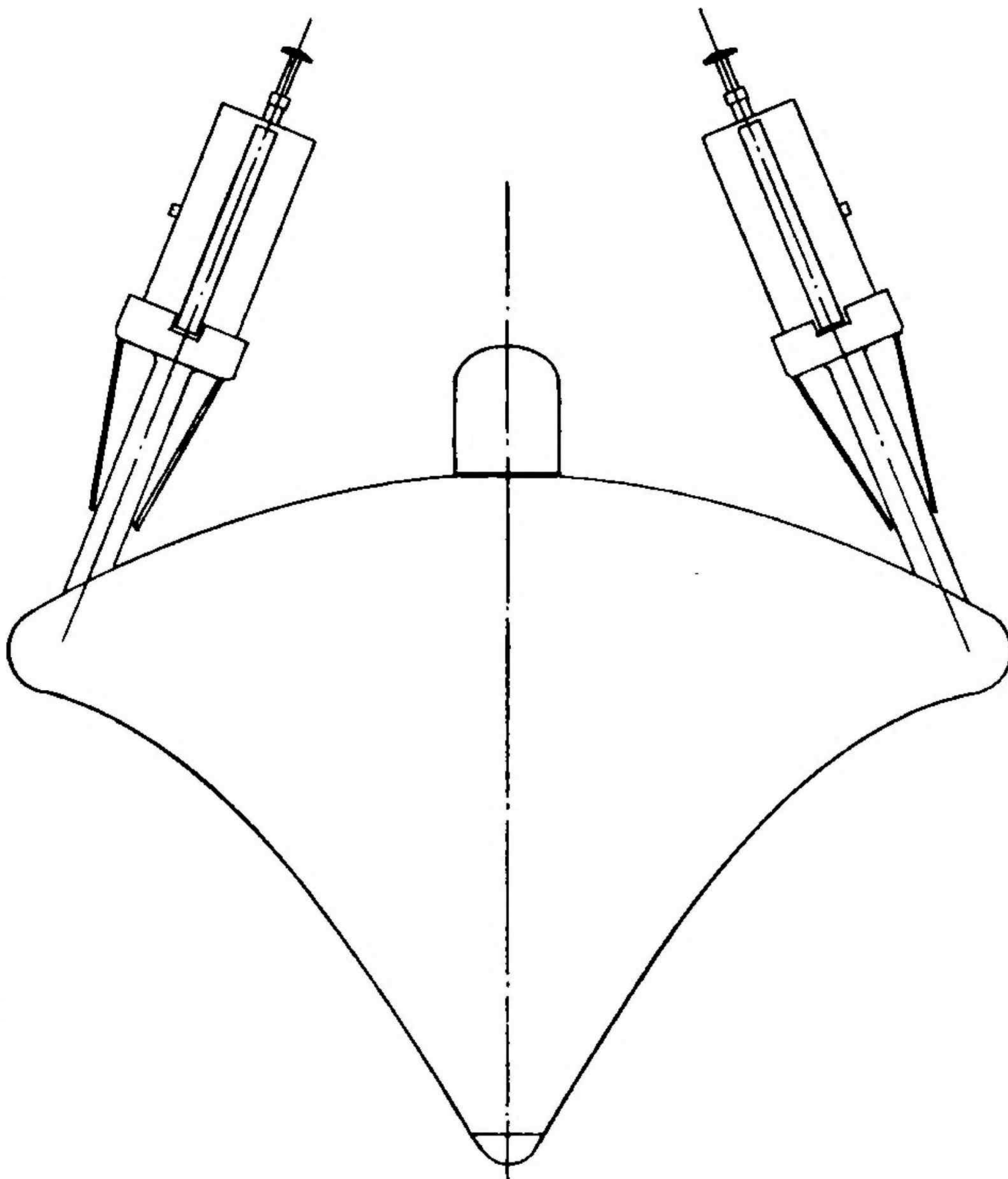
Figure 11 The spacecraft at entry into the atmosphere
