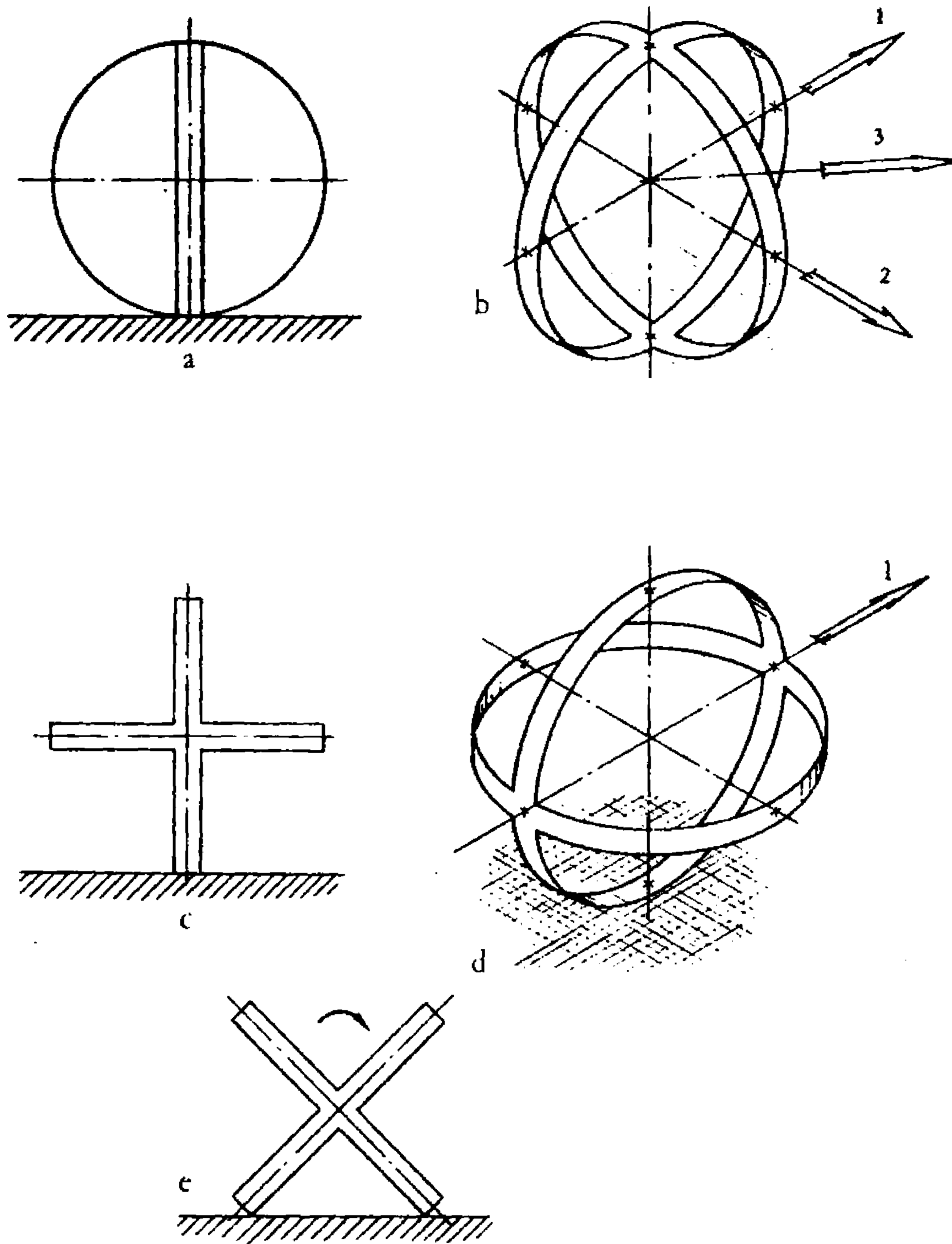
Figure 17 Characteristic positions of "crossed wheels"
