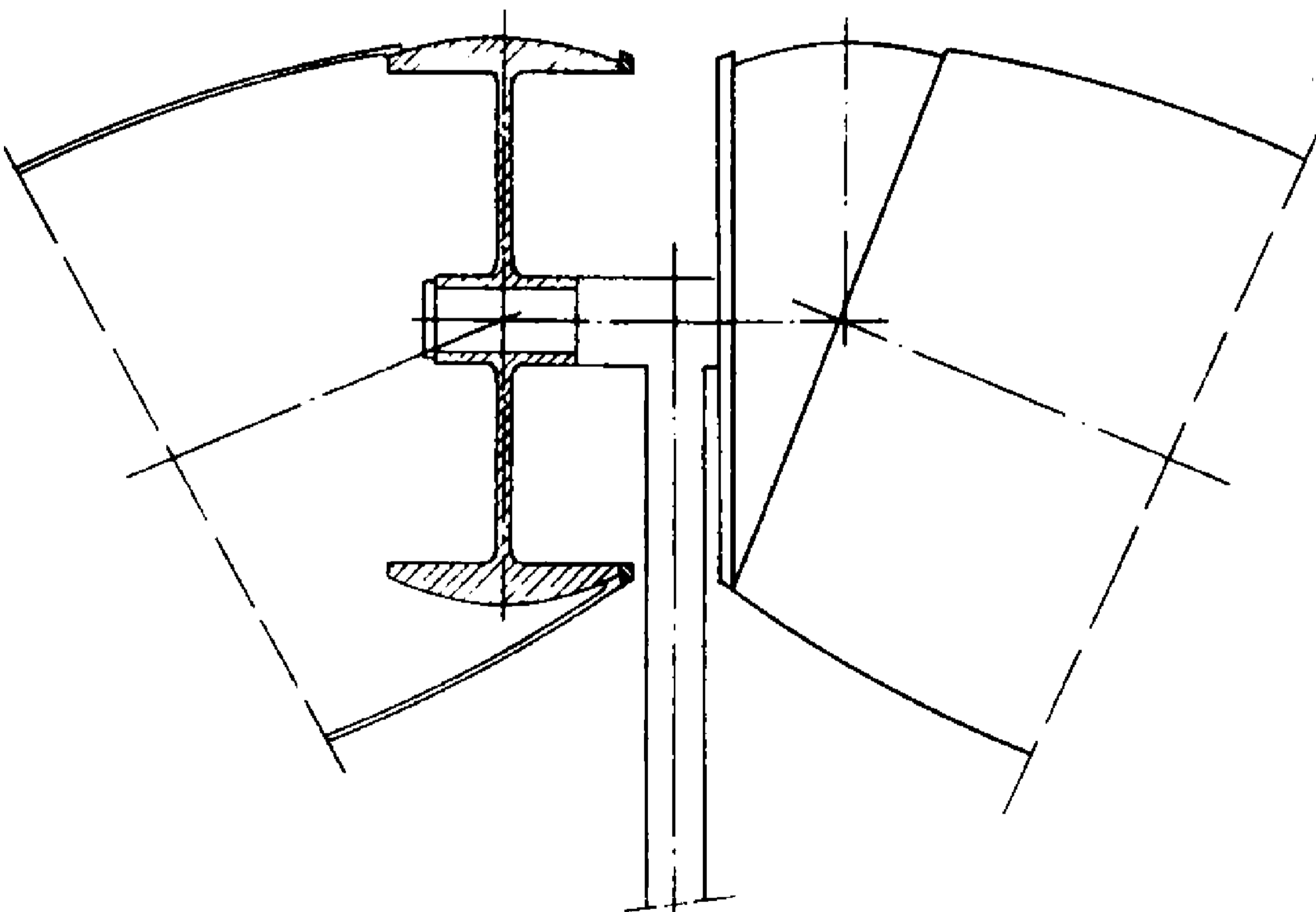
Figure 18 Support principle of the wheel segments
