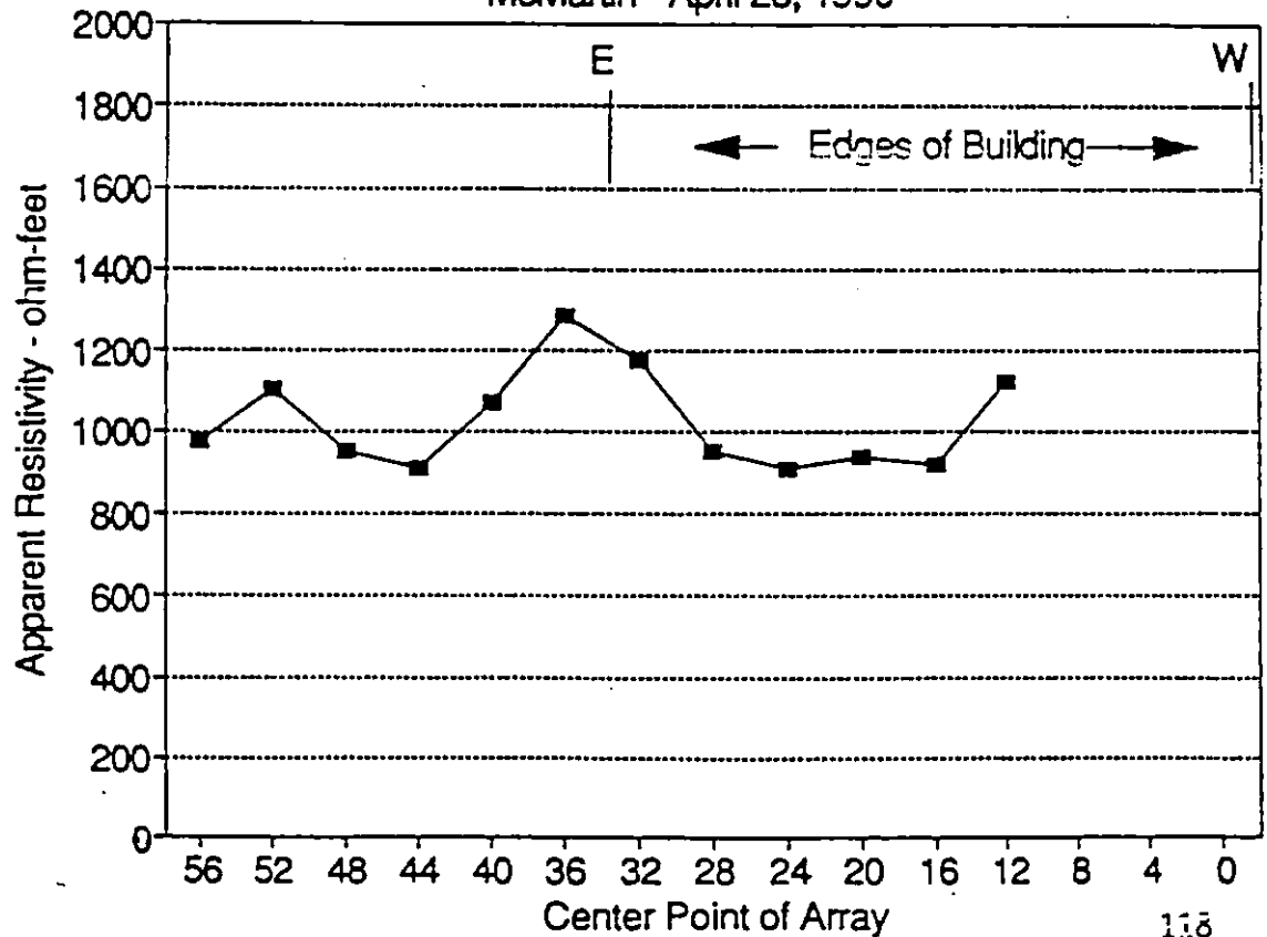
Electrical Resistivity Profile McMartin - April 28, 1990
